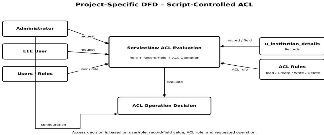
Figure 4.1: Solution architecture – ServiceNow Script-Controlled ACL.
